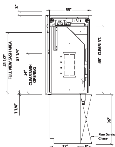
SECTION VIEW
